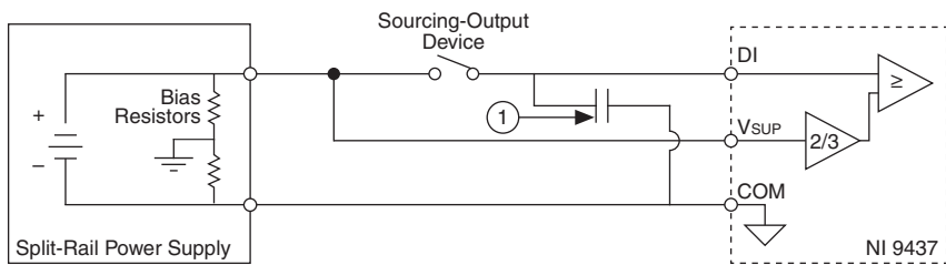
Figure 4. Capacitance Discharge
