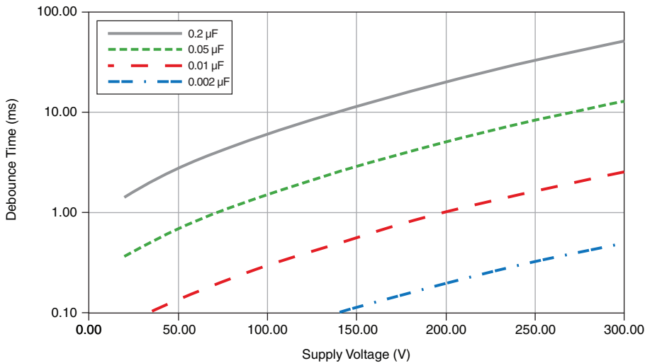
Figure 5. NI 9437 Turn-Off Time
